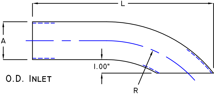
SHORT TAILPIPS O.D., INLETS
